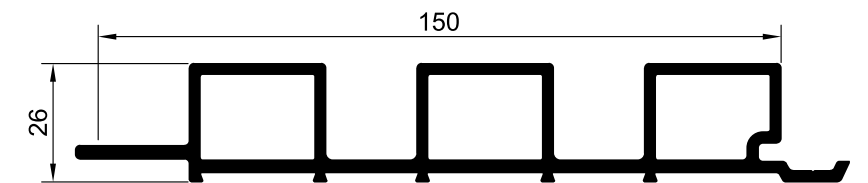
RIBBON (ÇİFT RENK) LINEAR 150x26 MM INTERIOR 280 CM EXTERIOR 280 CM/320 CM
