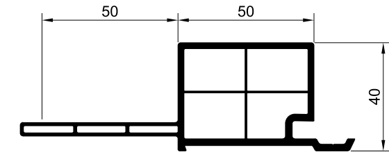
KARYA LINEAR 100x50 MM INTERIOR 280 CM EXTERIOR 280 CM/320 CM
