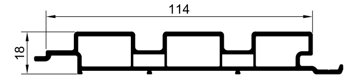
LINE LINEAR 114x18 MM INTERIOR 280 CM EXTERIOR 280 CM/320 CM
