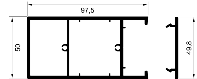
BAFFLE LINEAR 100x50 MM INTERIOR 280 CM EXTERIOR 280 CM/320 CM
