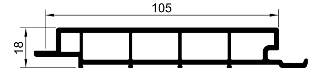
SOLID LINEAR 105x18 MM INTERIOR 280 CM EXTERIOR 280 CM/320 CM
